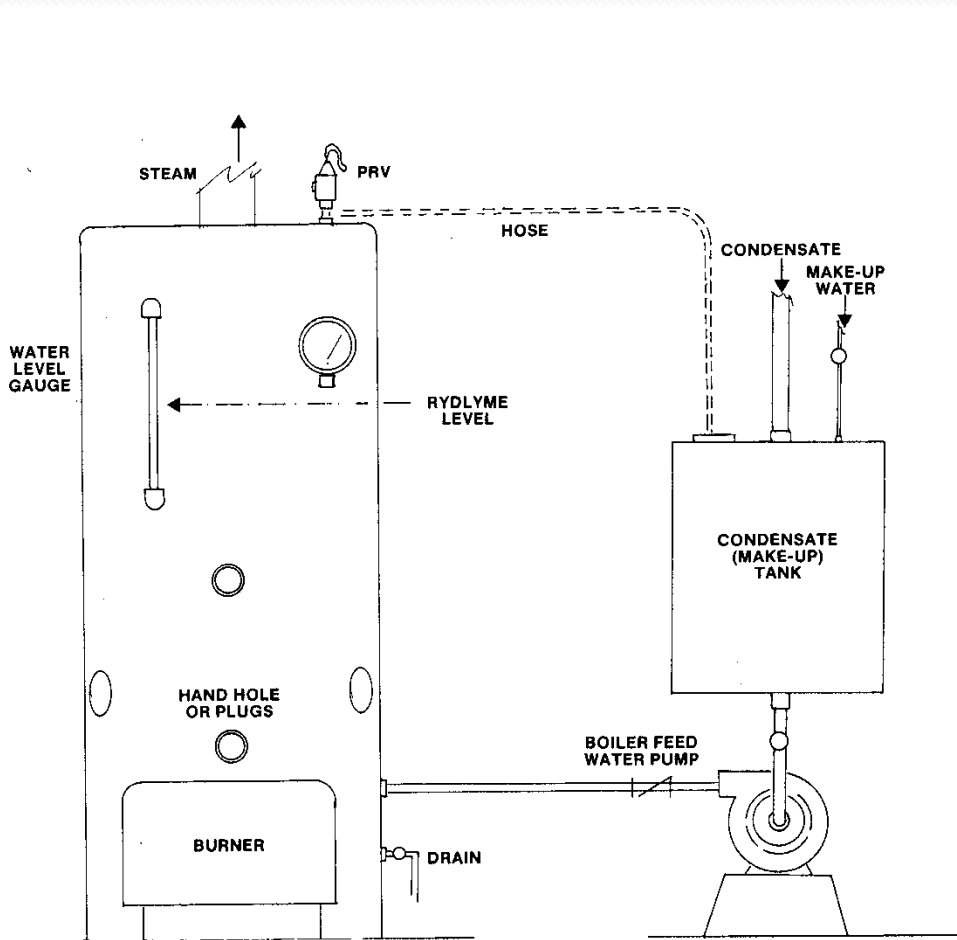
SMALL (UNDER 25 HP), HIGH PRESSURE STEAM BOILERS
